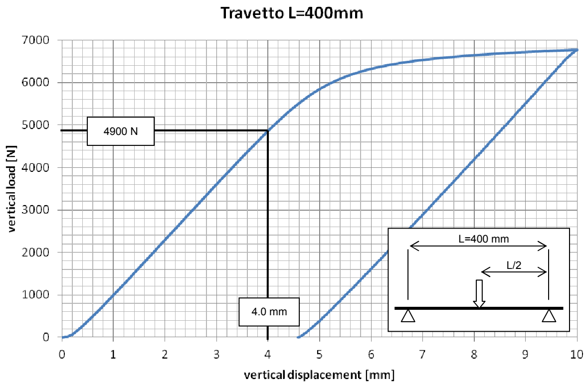
Fig. 2: test graph, load to 10mm and unload to 0 Newton.
