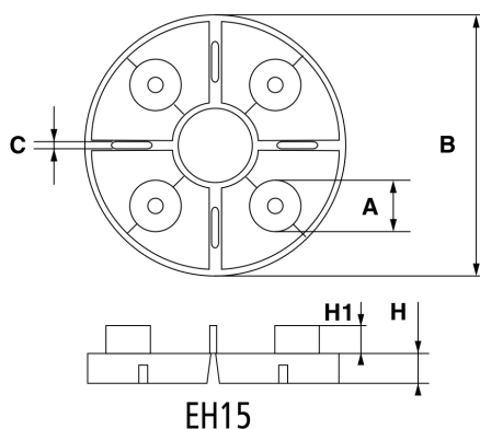
Figure 2 Typical "EH15" support specimen.
