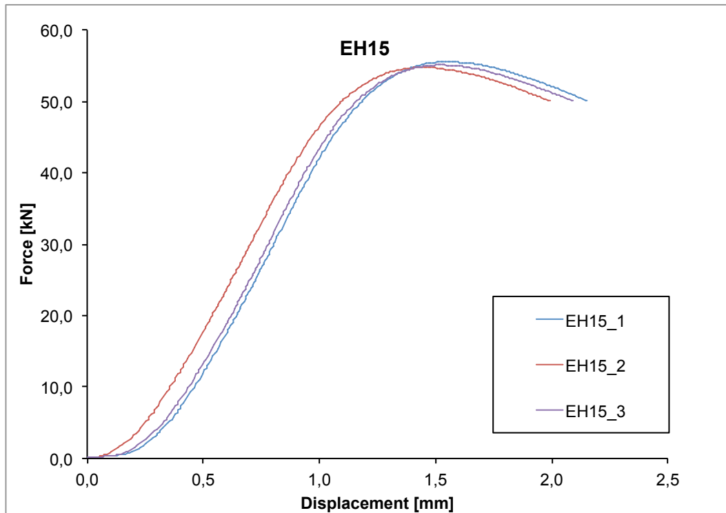
Figure 1 Diagram force versus displacement of testing machine's crossbar for "EH15" support specimen.
